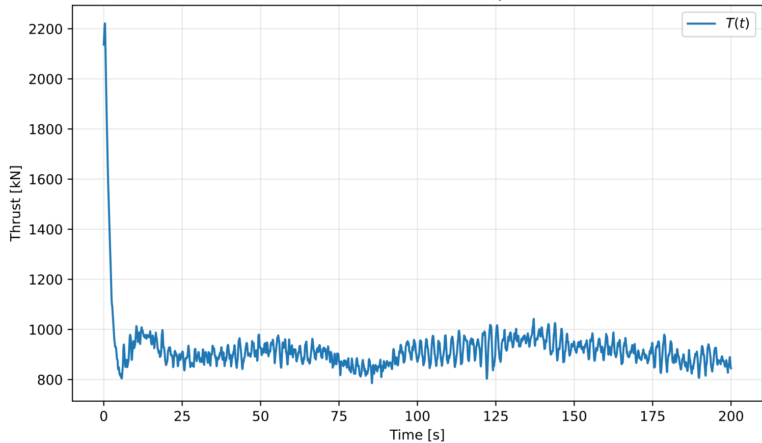
Turbulent wind: thrust response
